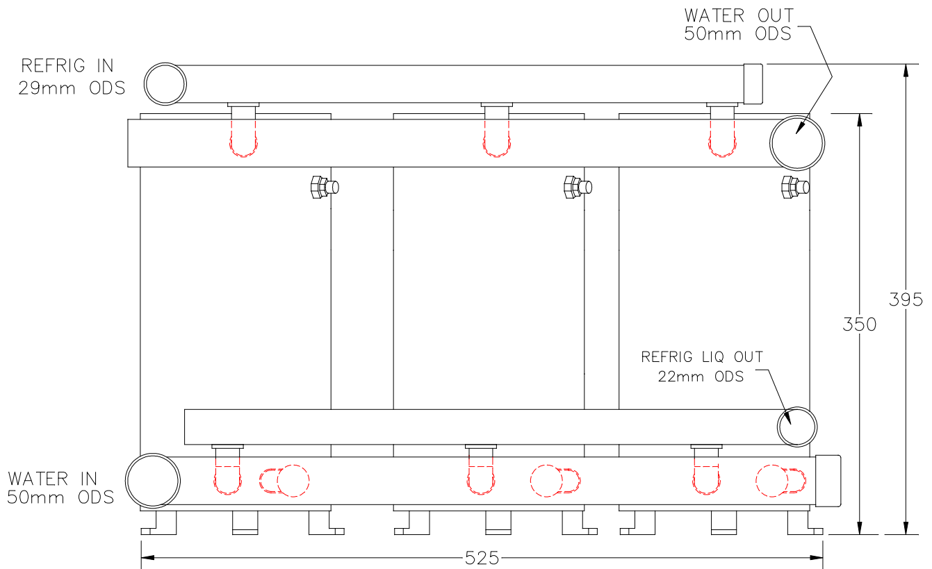
SIDE VIEW
