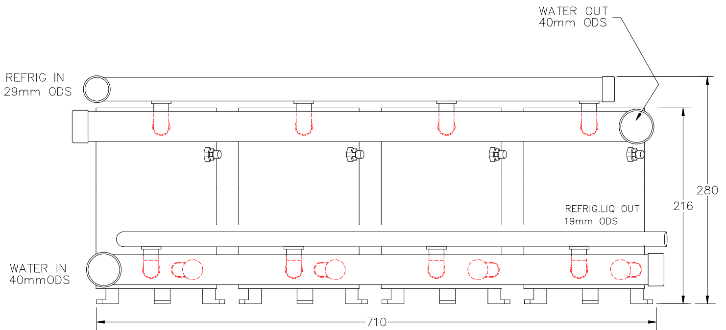
SIDE VIEW
