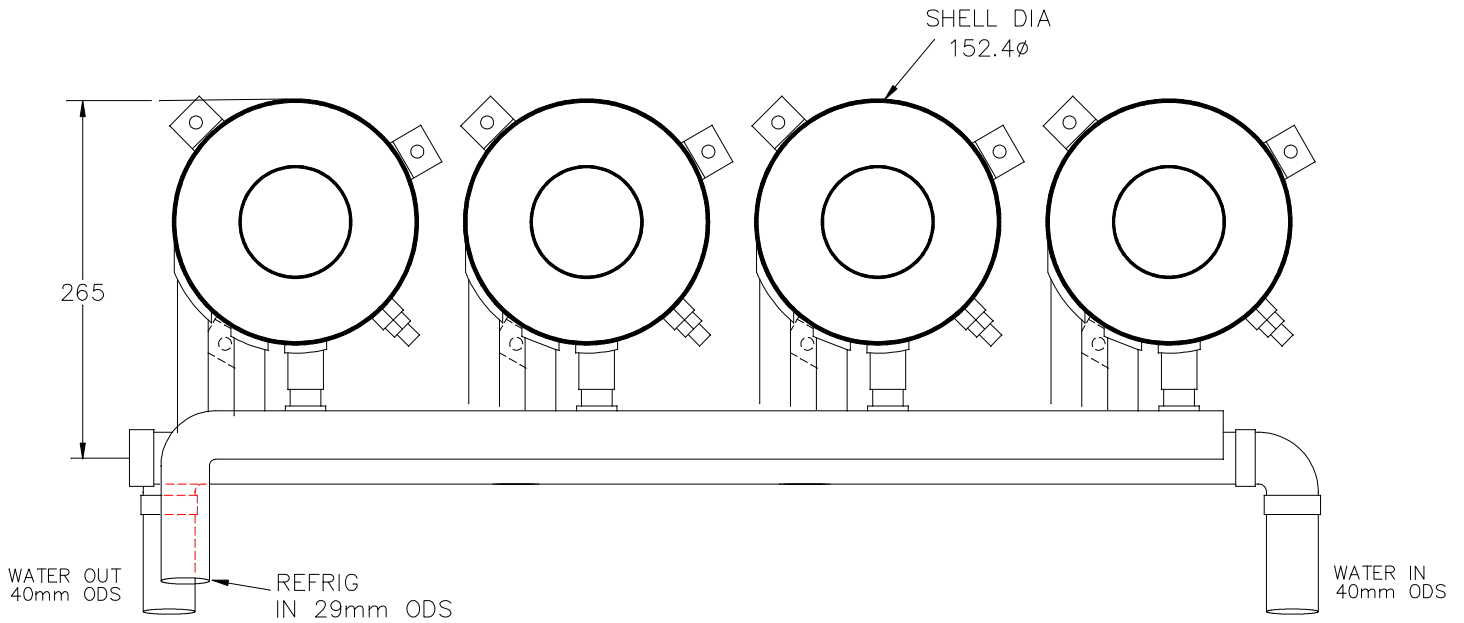
TOP VIEW
