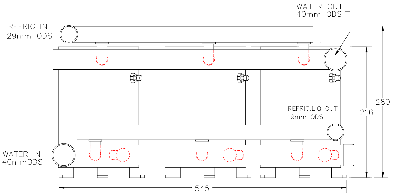
SIDE VIEW
