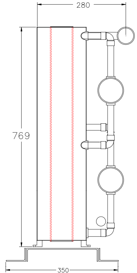
END VIEW
