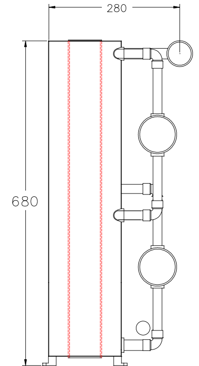
END VIEW
