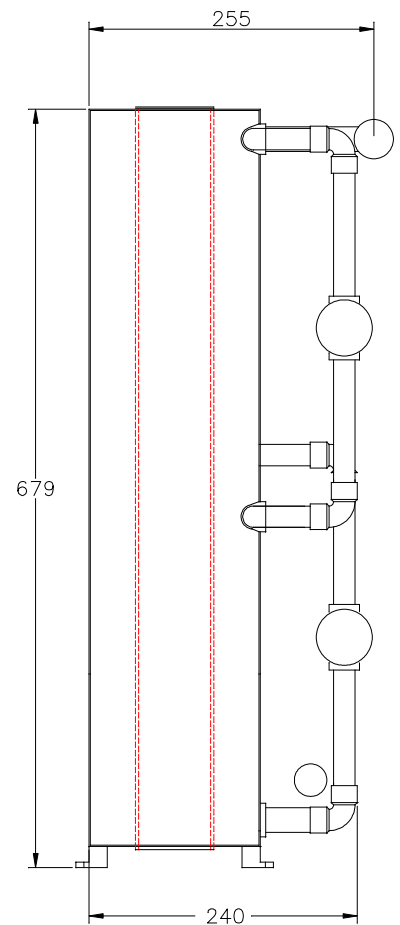
END VIEW
