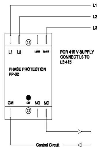
WIRING DIAGRAM PP-02 (380/415 VAC 50/60 HZ)
