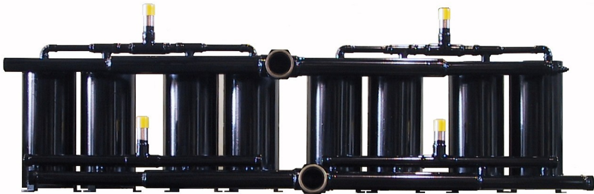
Aqua Systems Model S-6R/8H-2R1WC water cooled replacement condenser assembly for 50TR chiller with two refrigeration systems
