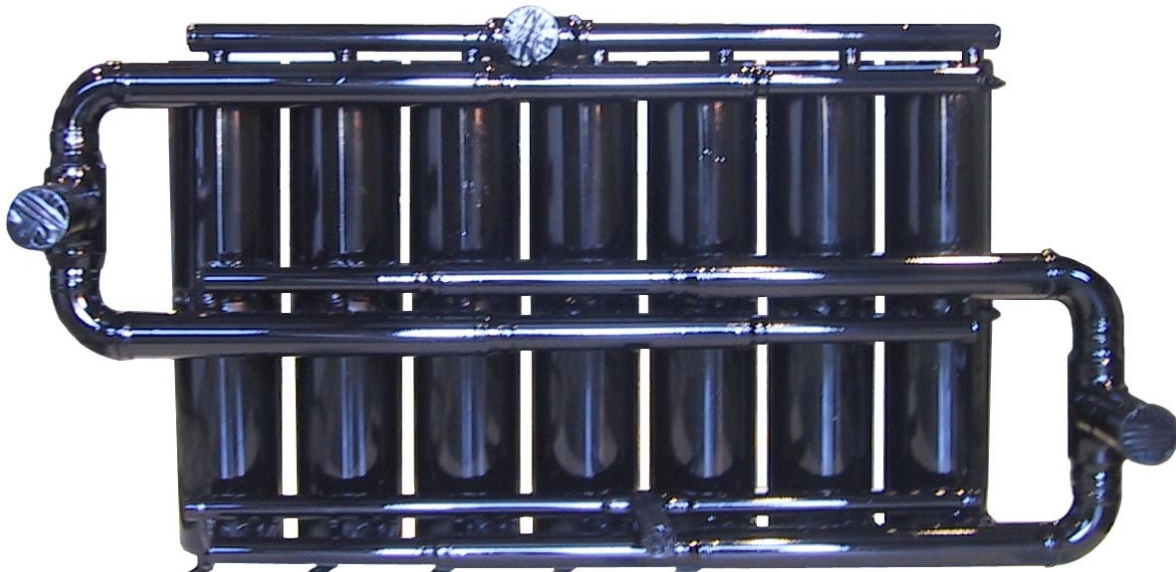
Aqua Systems Model S-6/14HV water cooled condenser assembly for 85TR liquid chiller
