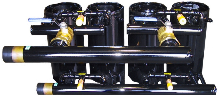
Aqua Systems Model S-6R/8H-2R1WC water cooled replacement condenser assembly for 50TR chiller with two refrigeration systems
