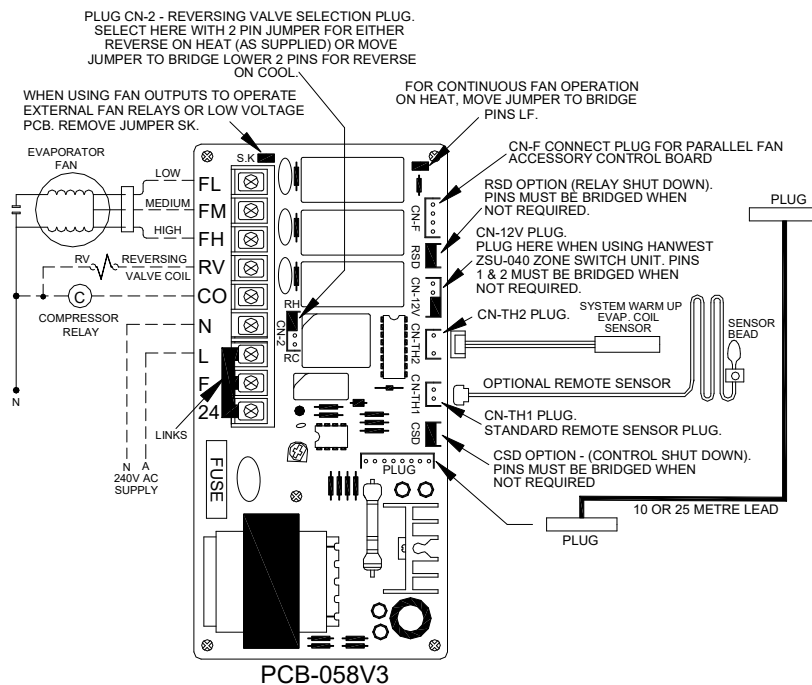
PCB-058V3 connection layout (FIG 3)
