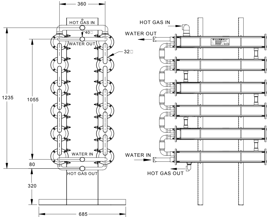
DISCHARGE DE-SUPERHEATER FOR AMMONIA REFRIGERATION SYSTEM. MODEL ADSH-6/2.
