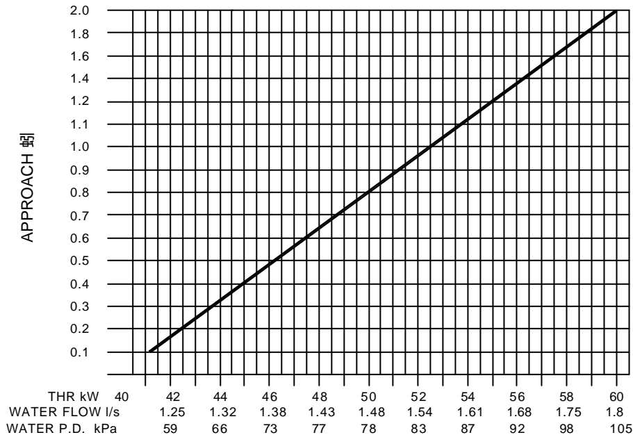
PARALLEL WATER FLOW MODELS S-6/2 S-6R/2 CN6/2
