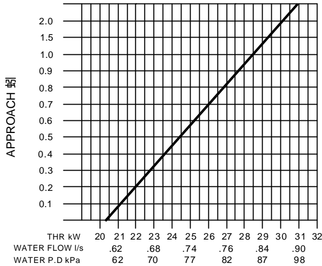
PARALLEL WATER FLOW MODELS S-6 S-6R CN6
