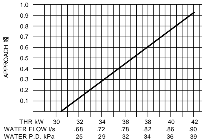
PARALLEL WATER FLOW MODELS S-5/2 S-5R/2 CN5/2
