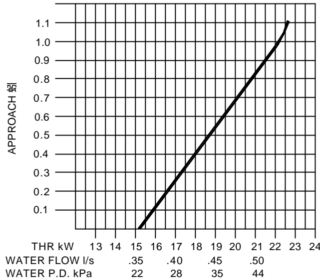
PARALLEL WATER FLOW MODELS S-5 S-5R CN5
