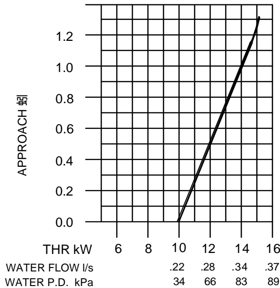
SERIES WATER FLOW MODELS S-3 S-3R CN3
