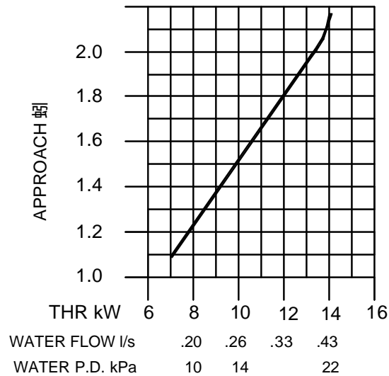
PARALLEL WATER FLOW MODELS S-3 S-3R CN3
